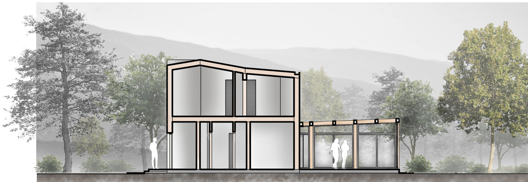
REZ C-C'
