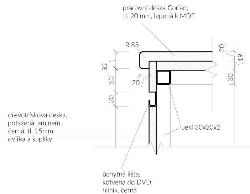
DETAIL A 1:5
