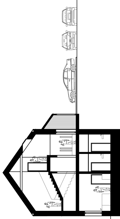
REZ AA
