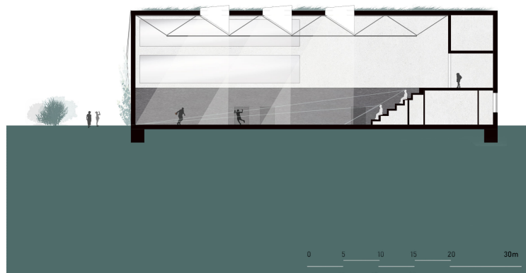
REZ C-C'
