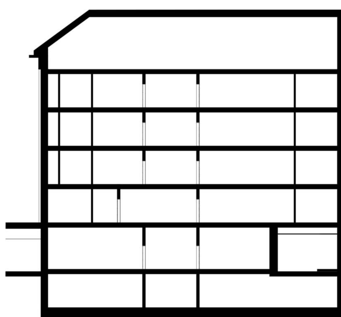
SECTIONS M1:200
