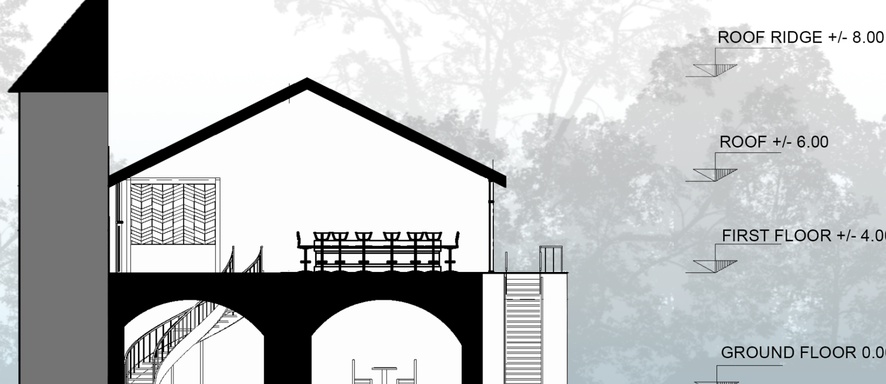
SEC. A - A'
