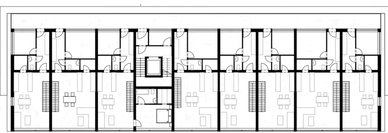
SECOND FLOOR - maisonette floor B
