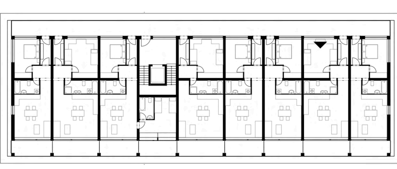
THIRD FLOOR - single storey
