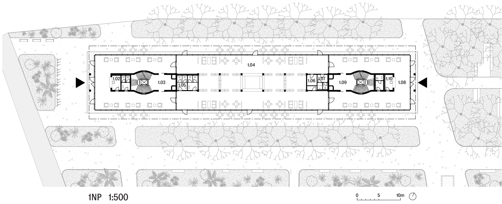
1NP 1:500
