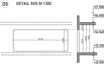
05 DETAIL 505 M 1:100
