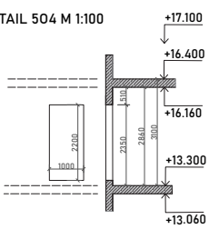
04 DETAIL 504 M 1:100
