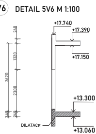
V6 DETAIL 5V6 M 1:100
