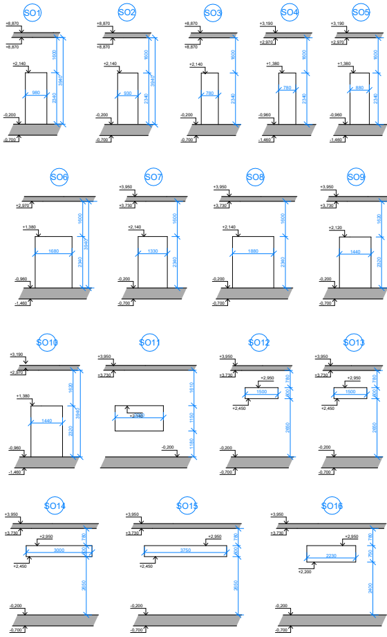
DETAILY M 1:20
