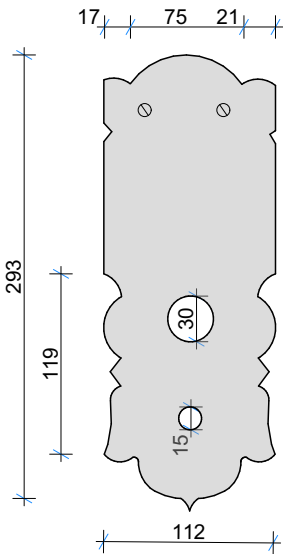
DETAIL M 1:5
