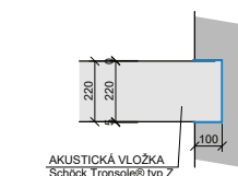
DETAIL 1 1:20
