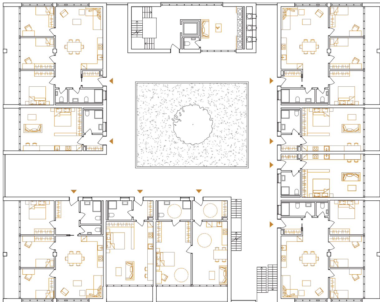
2NP + 3NP
